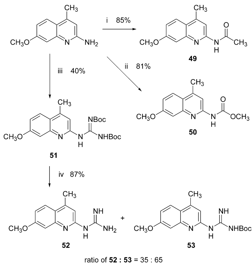
Scheme 2. The synthesis of the quinoline derivatives. Reagents: (i) acetic anhydride, TEA, cat. DMAP in \text{CH}_2\text{Cl}_2 ; (ii) methyl chloroformate, TEA, \text{CH}_2\text{Cl}_2 ; (iii) di-Boc- N -triflylguanidine, TEA, \text{CH}_2\text{Cl}_2 ; (iv) 5% TFA/ \text{CH}_2\text{Cl}_2 .
