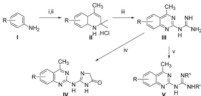
Scheme 1. General synthetic method for analogues in the quinazoline series. R = alkyl, alkoxy. Reagents: (i) iodine/acetone, reflux; (ii) HCl gas; (iii) cyanoguanidine; (iv) ethyl bromoacetate/DMF or glycine/water reflux; (v) acyl anhydride/DMSO.
